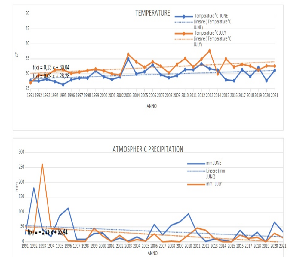
Figure 2: temperature and atmospheric precipitation changes
